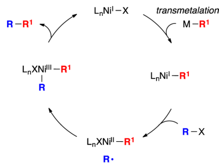
Figure 1. Outline of one of the possible mechanisms for nickel-catalyzed cross-coupling of unactivated alkyl electrophiles: transmetalation before oxidative addition.
